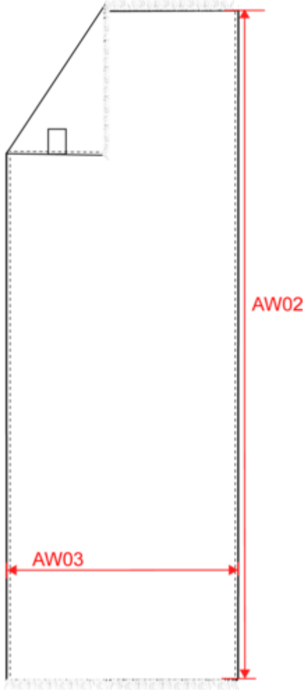
Dimensions (cm)
