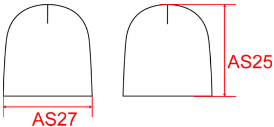
Dimensions (cm)
