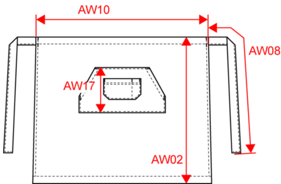
Dimensions (cm)
