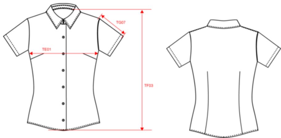
Dimensions (cm)
