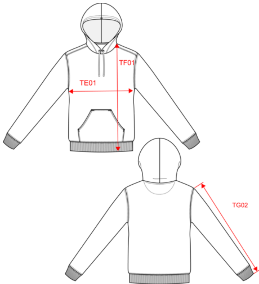
Dimensions (cm)
