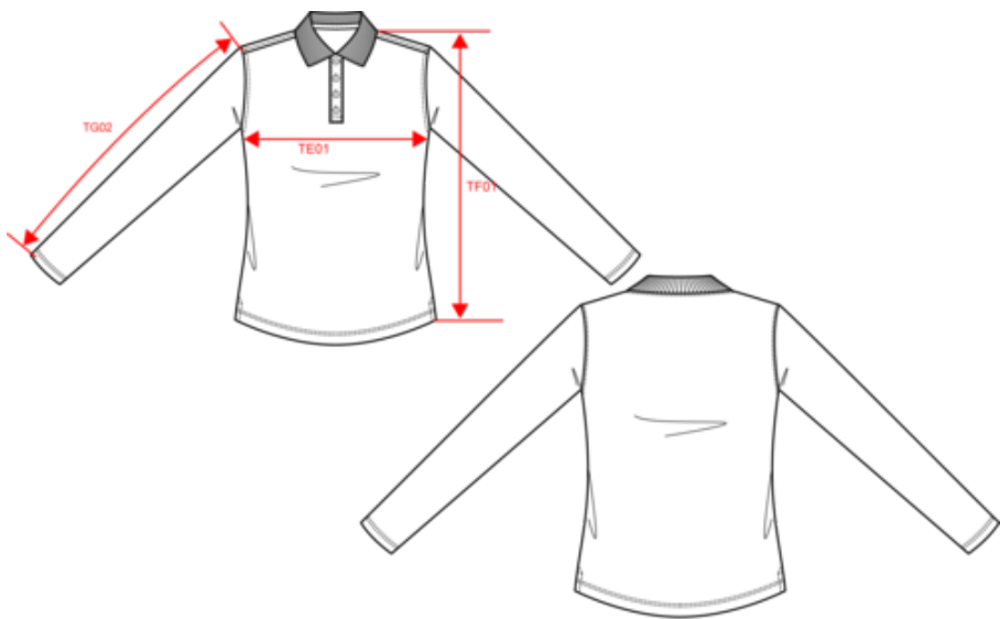
Dimensions (cm)
